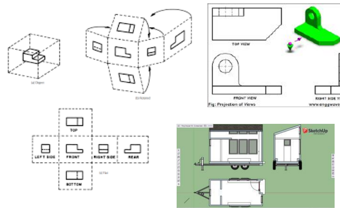
Orthographic drawing
